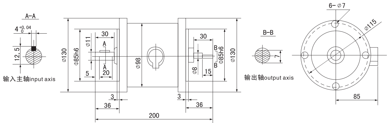
LLY101-X型超速开关外形及安装尺寸 LLY101-X overspeed switch Shape and mounting dimensions
